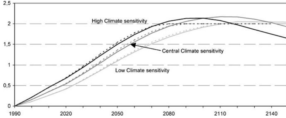
Figure 3. Global mean temperature increase for 3 climate sensitivities: in a cost-benefit analysis with Pure Preference for Climate Current Regime based on a desired 2°C target (full curve) and in a cost-efficiency analysis with a 2°C target (dotted curve).
