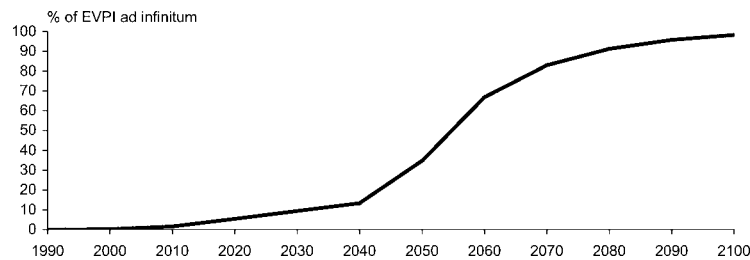
Figure 2. Expected Value of Perfect Information with respect to the date of resolution of uncertainty on climate sensitivity. Information value raises brutally after 2040, that means there is a significant interest in revealing this value before this date [17].
