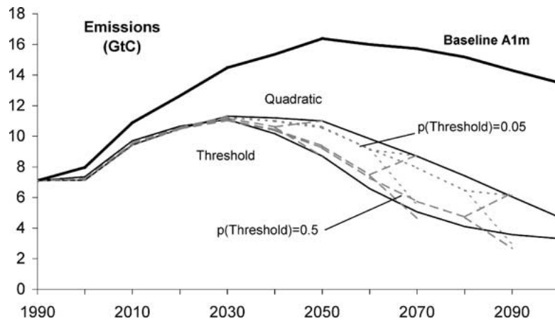
Figure 10. Emissions paths for different subjective probabilities of the threshold function with learning. Threshold function probability: 0% for the upper thin black line; 5% for the dotted grey line, 50% for the dashed grey line; 100% for the lower thin black line. Learning occurs in 2040, 2060 and 2080.
