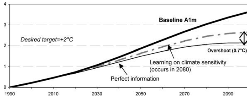
Figure 4. Comparing the cost of misestimating belief on climate change damages and climate dynamics. In all cases, climate sensitivity has a high value. Global mean temperature increase for baseline case (bold black curve), for optimal strategy with perfect information (thin black curve) and for optimal strategy with learning on climate sensitivity (grey curve).
