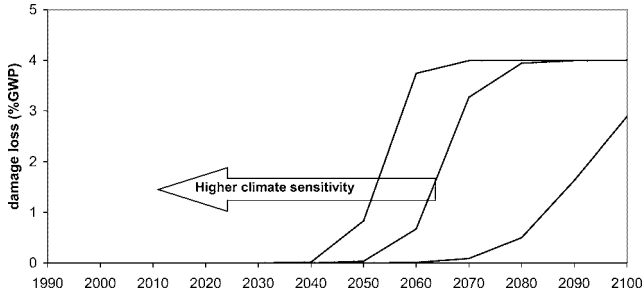
Figure 7. Depending on the value of climate sensitivity, in the case of singularities around a +2°C warming threshold, abrupt shifts (in the baseline case) occur sooner as climate sensitivity is higher.
