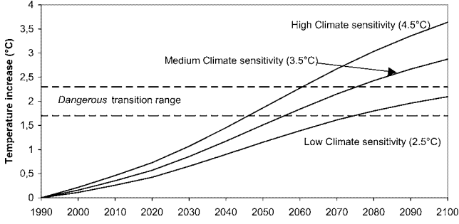
Figure 6. Global mean temperature rise with respect to 1990, with A1 emission baseline and three values for climate sensitivity.
