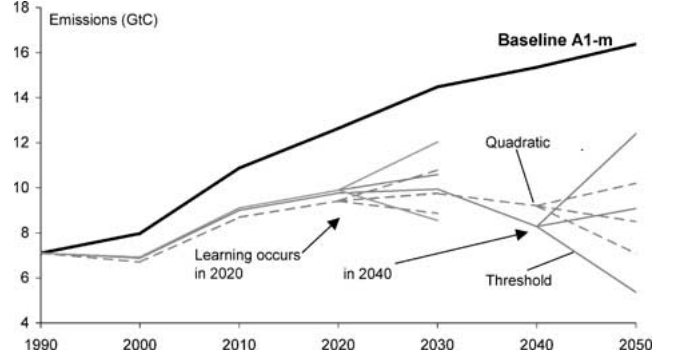
Figure 8. Emissions path for quadratic (dashed grey curves) and threshold (full grey curves) damage functions and learning on climate sensitivity in 2020 or 2040.
